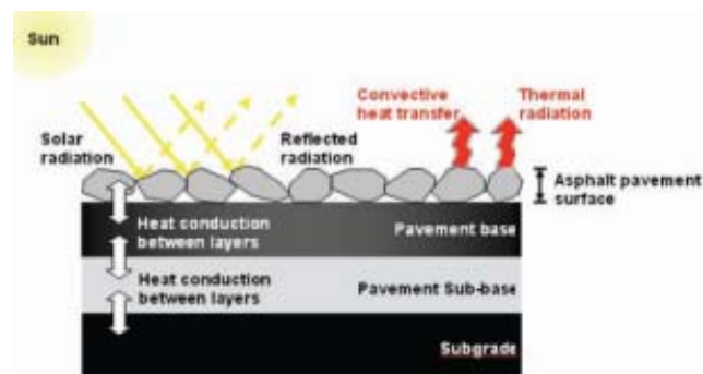
Figure 9: Heat Transfer In Asphalt Road Pavement
